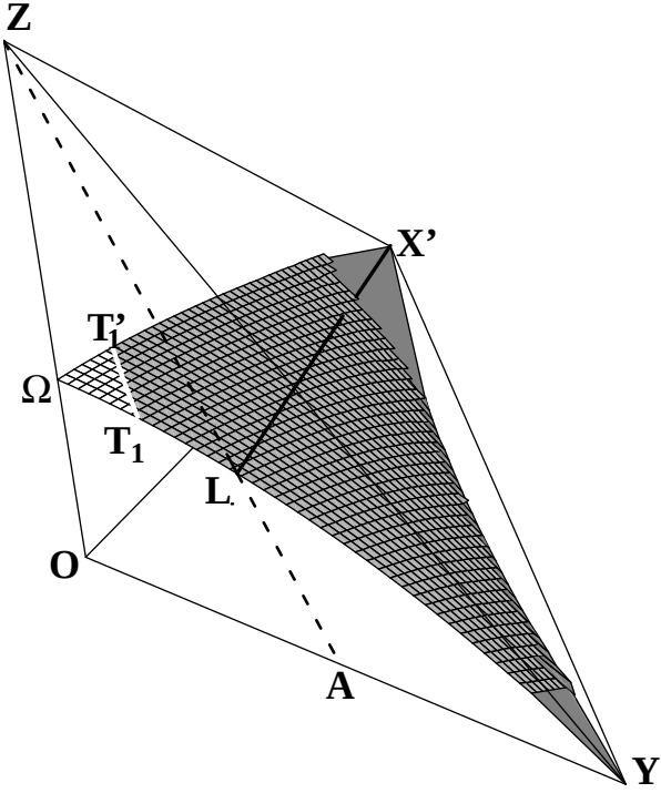
Figure 11: The transition surface between the two Haldane phases with different topological order in the [-, +, +] sector. The dark part of the surface corresponds to the zero-gap critical part. All points of the mesh are DMRG results. Our DMRG results are not accurate in the vicinity of ferromagnetic ( X' ) or antiferromagnetic ( Y ) decoupled chains. The grey areas are simple extrapolations. The critical part of the surface is bounded through the tricritical T_1T'_1 white line. On T_1T'_1\Omega the transition is first order with two degenerate ground-states and finite gap. The cut by the plane ALZX' corresponds to the “Zig-Zag chain” model (cf. Fig. 6 in section IV). The straight line LX' lies in the critical surface.
