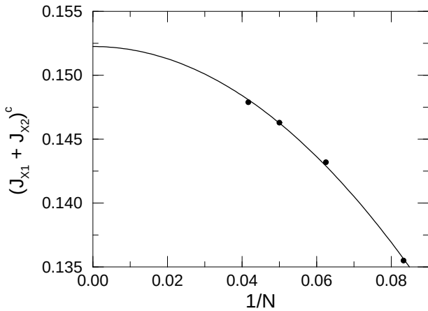
Figure 9: Critical value of S = J_{X1} + J_{X2} for which the difference \delta between the two lowest excited states vanishes, as a function of 1/N , for finite chains with periodic boundary conditions. We follow the transition line \Omega LY determined through DMRG in the OYZ plane (Fig. 10). A quadratic extrapolation gives (J_{X1} + J_{X2})^c \approx 0.152 in the thermodynamic limit, fixing the position of T_1 on the transition line.
