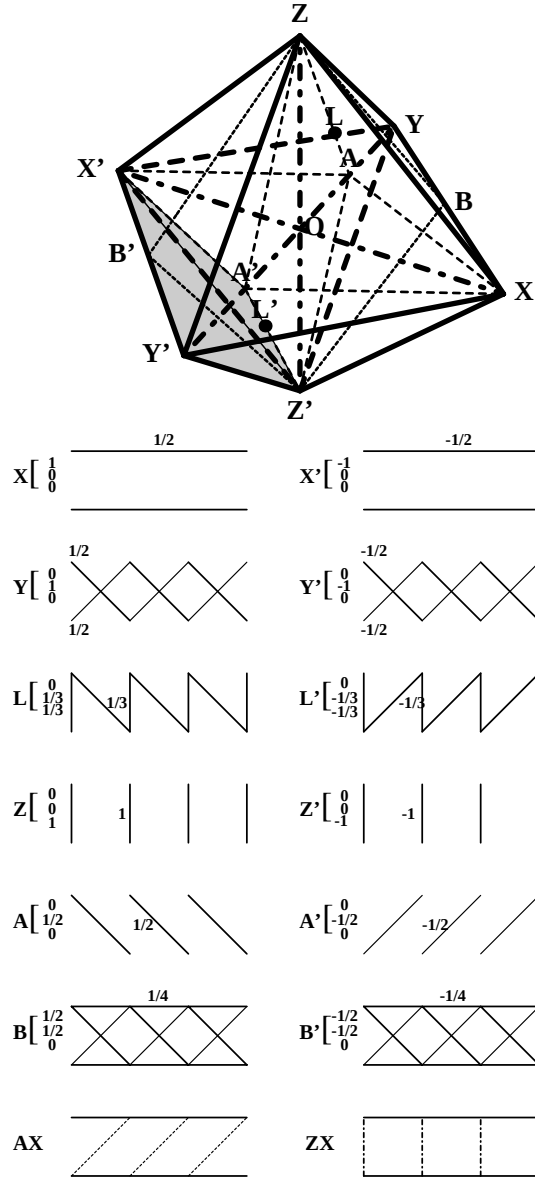
Figure 2: The regular octahedron inscribed in a sphere of radius 1, representing the parameter-space of our Hamiltonian [Eq. (1)] with the energy scaling of Eq. (3). Some remarkable points with their \{x, y, z\} coordinates are listed: the spin- \frac{1}{2} Heisenberg antiferromagnetic (X,Y,L) or ferromagnetic (X',Y',L') chain, products of independent dimers (A,Z) or triplet pairs (A',Z'), the usual ladder (AX and ZX segments) etc... The "Zig-Zag" chain represented in Fig. 1 (a) corresponds to the surface of the irregular octahedron (AA',XX',ZZ'). In the gray volume, all interactions are negative (ferromagnetic).
