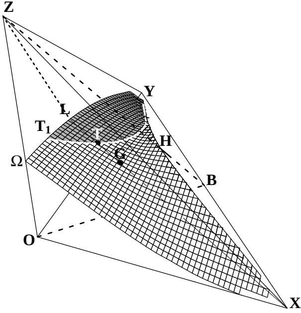
Figure 7: The transition surface separating the two gapped Haldane phases with different topological order in the [+,+,+] sector. Each point of the grid has been obtained through DMRG, keeping 30 states. The dark part of the surface is critical with vanishing gap and string-order parameters. The clear part corresponds to a first-order transition with finite gap and degenerate ground state. The white line which separates both parts of the surface thus appears as a tricritical line. The cuts of the surface through the planes XALZ, OBHZ, XYZ, and OYZ have been represented in Figs. 6, 7, 8 and 10 respectively. The straight line LTGX, joining L (one simple Heisenberg chain) to X (two decoupled Heisenberg chains) lies in the surface. The Majumdar-Ghosh point G corresponds to the intersection of this line with the OBHZ plane. Near X, our DMRG results are consistent with the exact result obtained from field theory (see text), i.e. the transition surface is tangent to the plane J_{\perp} = S = J_{X1} + J_{X2} .
