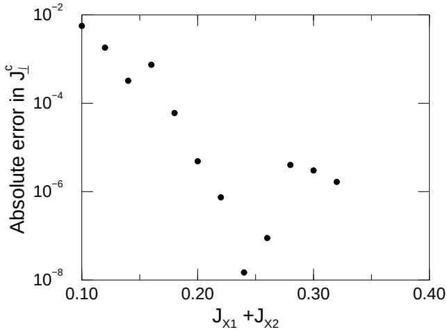
Figure 8: A test of accuracy of our DMRG scheme, with only 30 states kept, along the exact transition line LX. The accuracy is best (7 digits) near the Majumdar-Ghosh point G. It decreases drastically to 3 to 2 digits close to X (two decoupled Heisenberg chains) and also decreases when moving to L in the critical regime as the second-order transition becomes softer.
