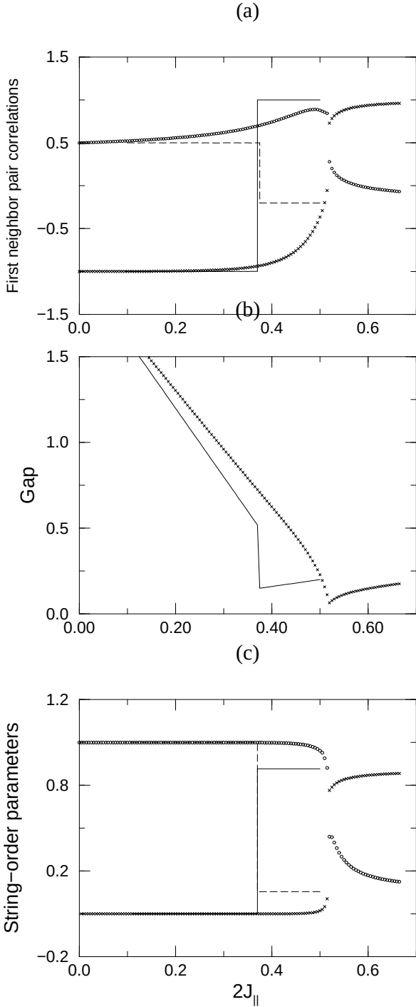
Figure 5: First order transition between Haldane phases with different topological order. (a) Pair correlation C_{\perp} along ZW (crosses) and ZB (full line); pair correlation C_{X1} along ZW (circles) and ZB (dashed line). (b) Gap along ZW (crosses) and ZB (full line). (c) String order parameter \tilde{O}_X along ZW (crosses) and ZB (full line); string order parameter \tilde{O}_{\perp} along ZW (circles) and ZB (dashed line).
