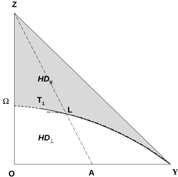
Figure 6: The transition line between the two Haldane phases with different topological order in the J_\parallel = 0 plane. L represents a simple spin- \frac{1}{2} antiferromagnetic Heisenberg chain and Y two decoupled chains. The heavy line YLT_1 is critical with zero gap. On T_1L (dotted line), the transition is first order. The dash-dotted line is a simple approximation to the critical line.
